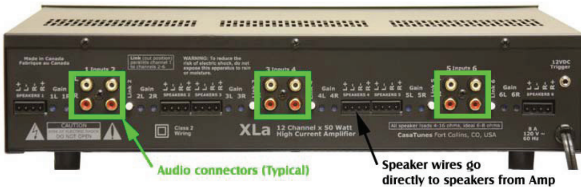
Amplifier
