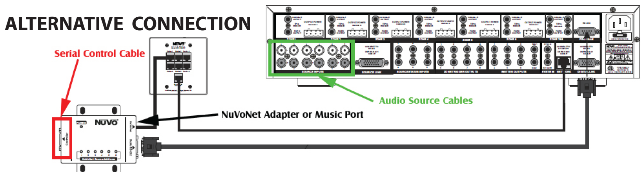
Nuvo controller (Grand Concerto shown) with NuVoNet/Music Port Adapter
